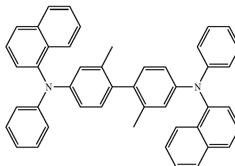
methylated-NPB
