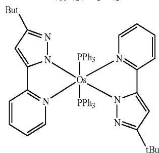
Os(bppz) 2 (PPh 3 ) 2
