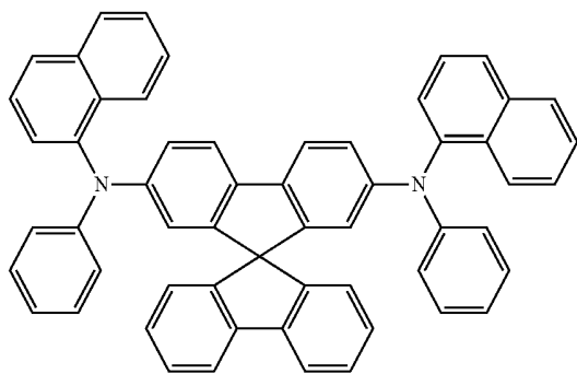
spiro-NPB
